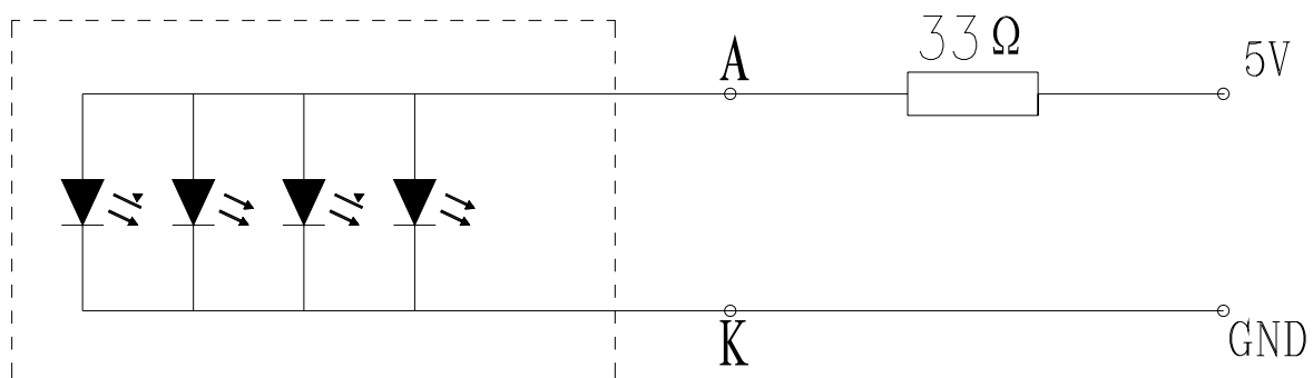
Test Circuit
