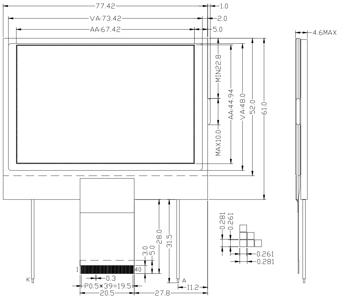
outline dimension
