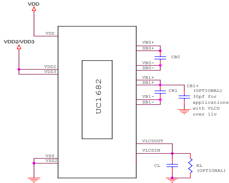
FIGURE 3: Reference circuit using internal Hi-V generator circuit
