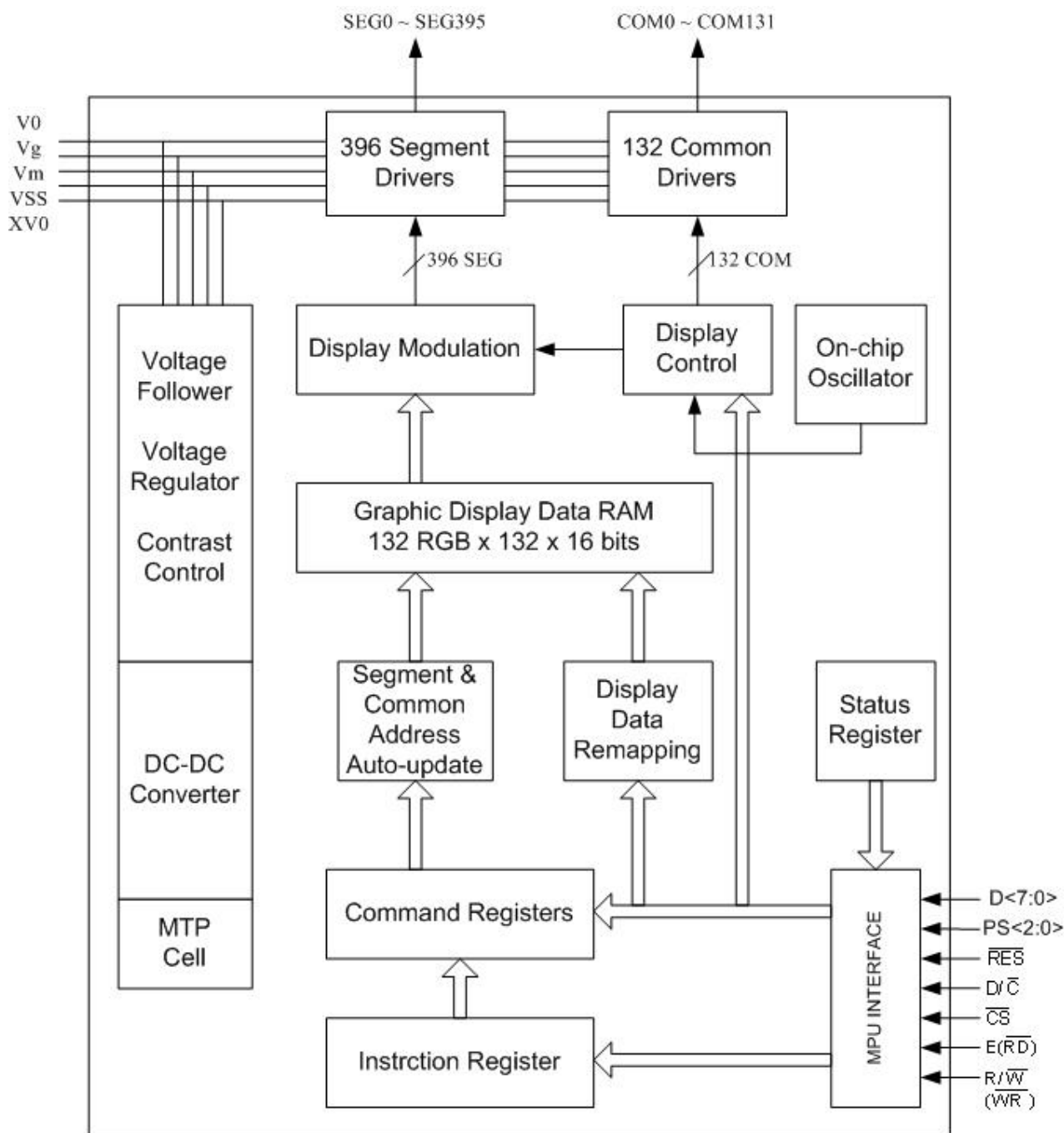
Figure 2 TLS8103 block Diagram
