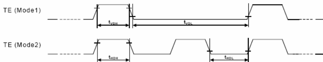
Figure18 Tear affection timing diagram
