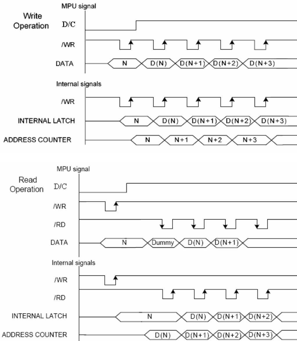
Figure17 Parallel interface pipeline data access
