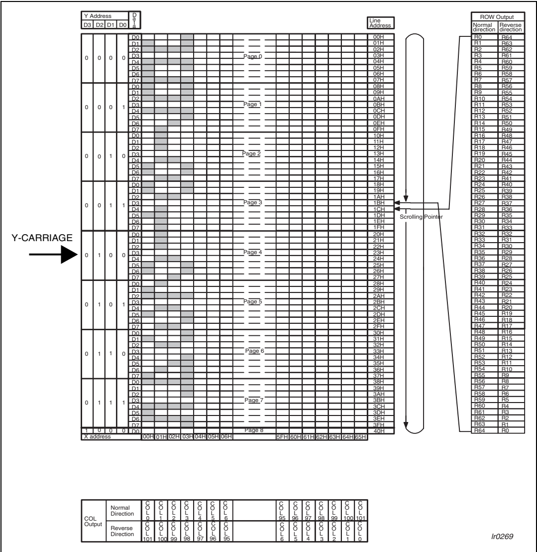
Figure 19. Memory rows vs. row drivers mapping ICON_MODE=0 and MUX 65
