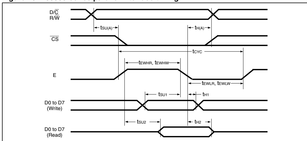
Figure 73. 68000-series parallel interface timing
