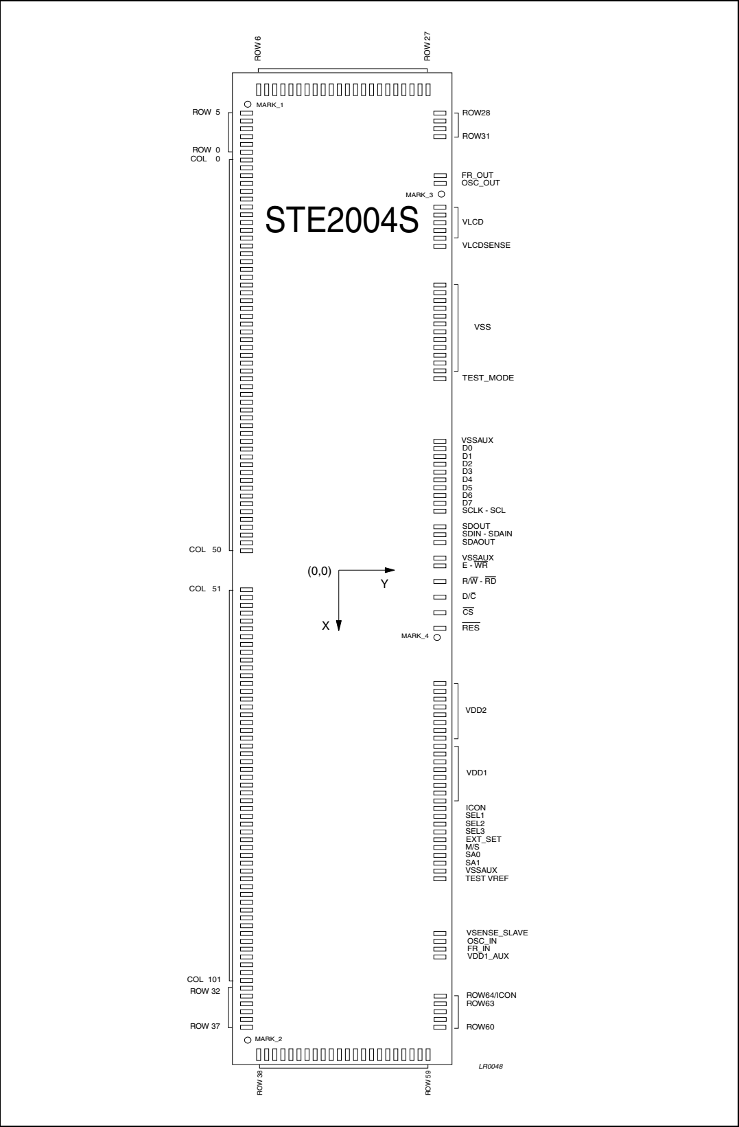
Figure 2. Chip mechanical drawing
