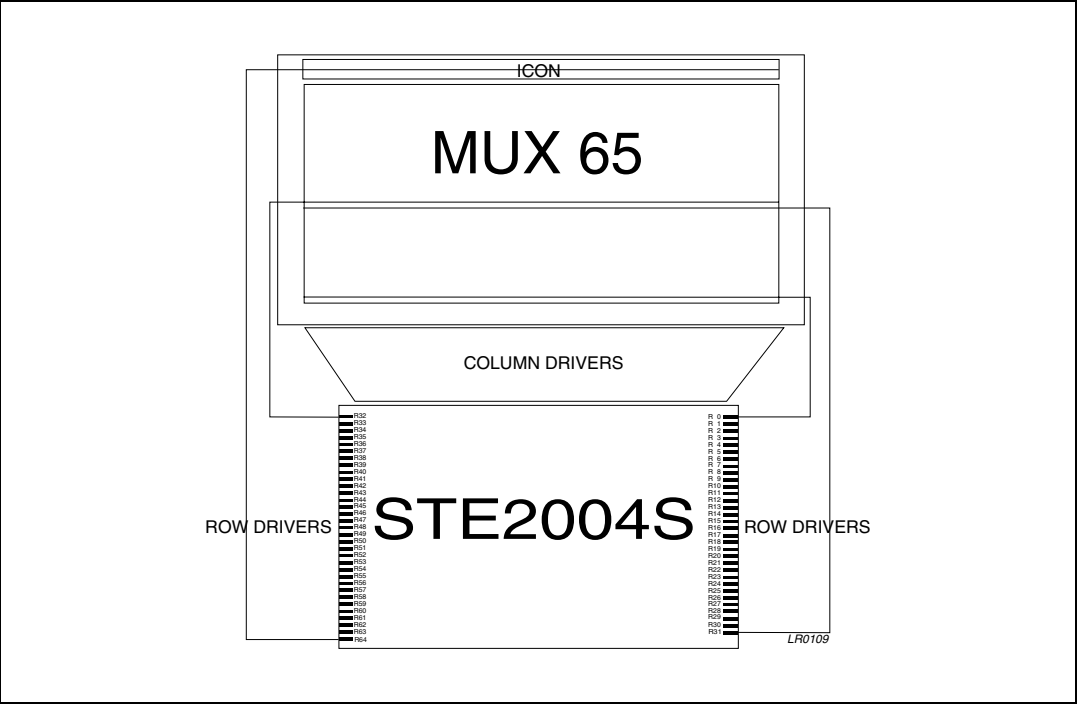
Figure 28. Row drivers vs. LCD panel interconnection in MUX65 mode
