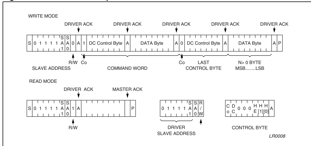
Figure 33. Communication protocol
