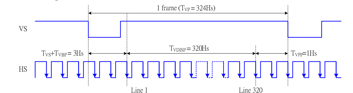
Fig. 9.9.11 RGB mode 2 vertical timing diagram
