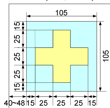
Alignment mark R (“+” type)
