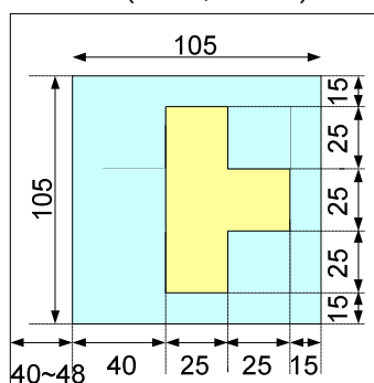
Alignment mark L ("T" type)
