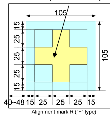
Alignment mark R (“+” type)
