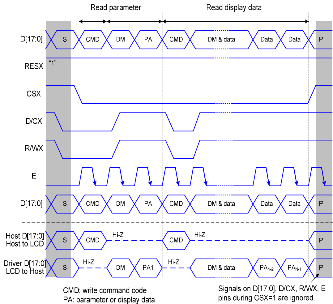
Fig. 9.3.4 6800-series parallel bus protocol, read data from register or display RAM
