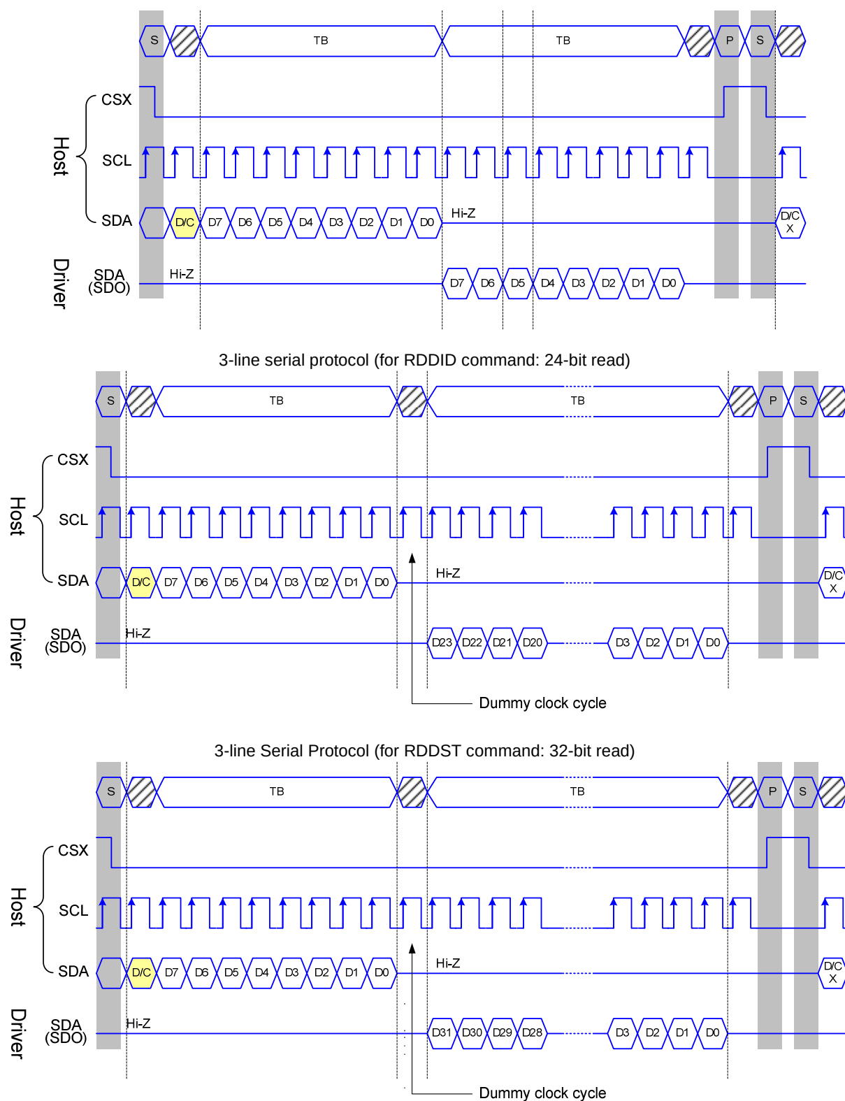
Fig. 9.4.4 3-line serial interface read protocol
