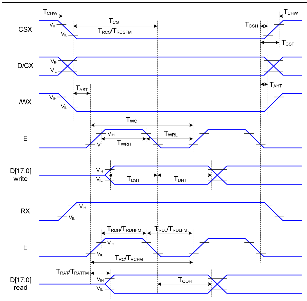
Figure 8.2.1 Parallel interface timing characteristics (6800-series MCU interface)
