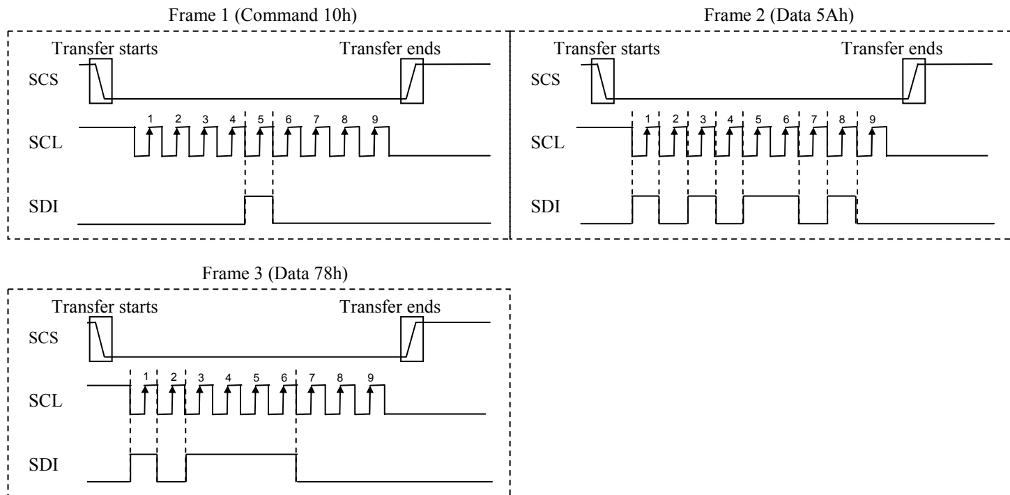
Example of 3-wires (9 bits)
