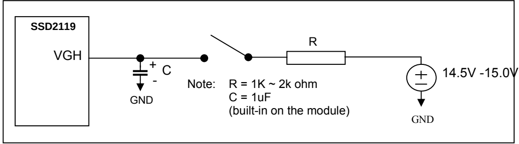
Figure 9-3: OTP circuitry
