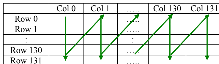
Figure 10-3 : Address pointer movement of vertical address increment mode
