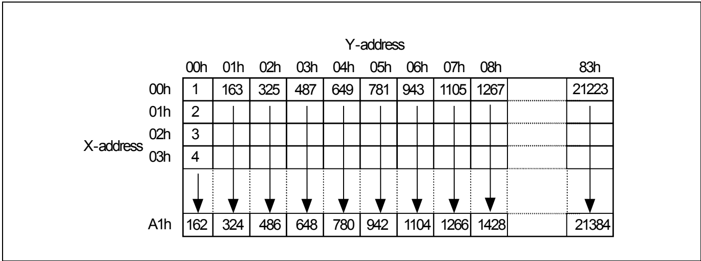
Figure 12. X address count mode
