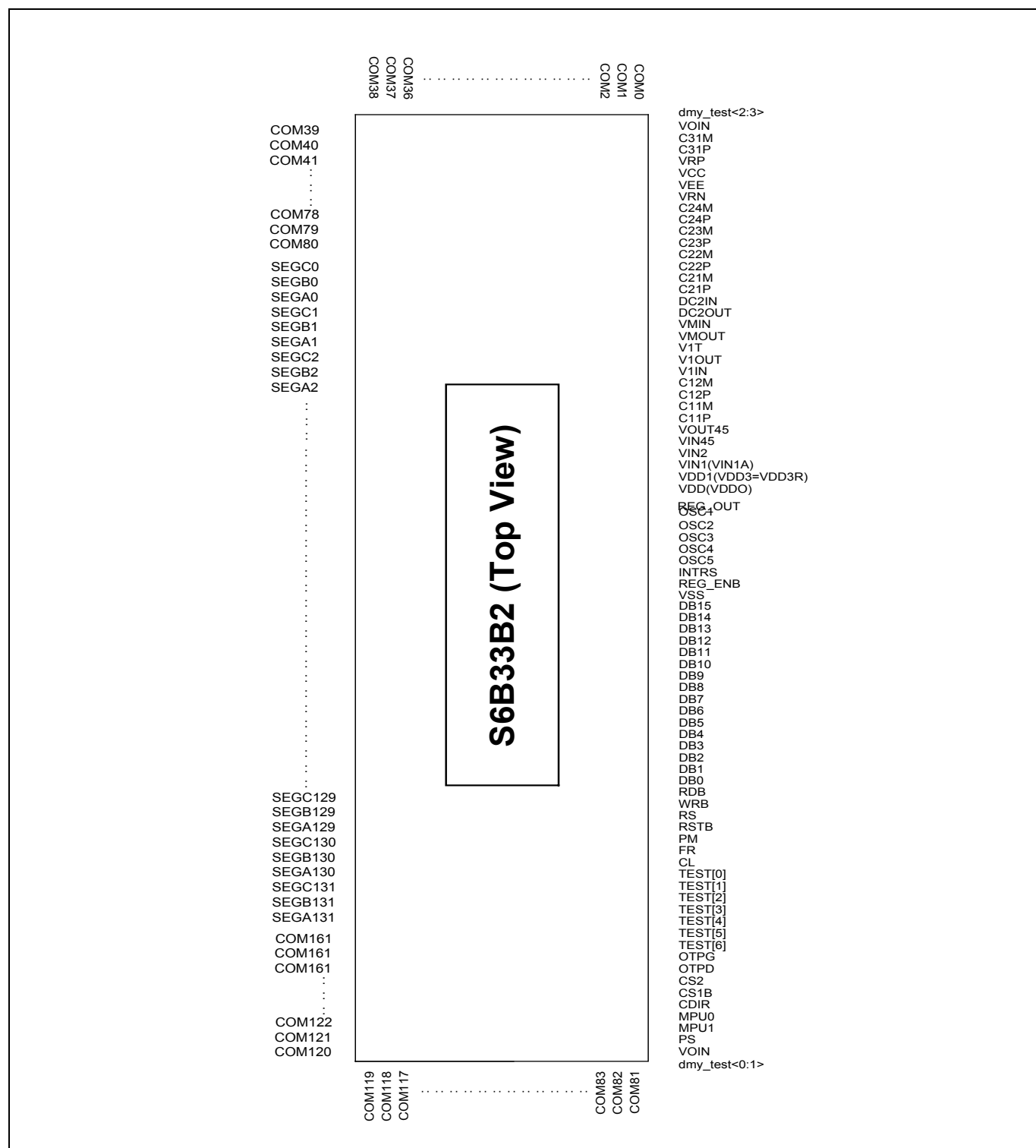
Figure 5. S6B33B2 Chip Pin Configuration
