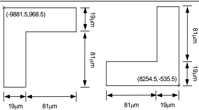
Figure 4. ILB Align Key Coordinate
