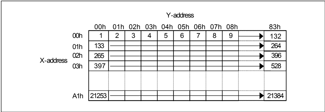
Figure 11. Y address count mode
