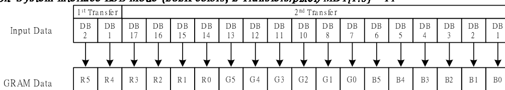
Figure3 16-bit System Interface Data Format
