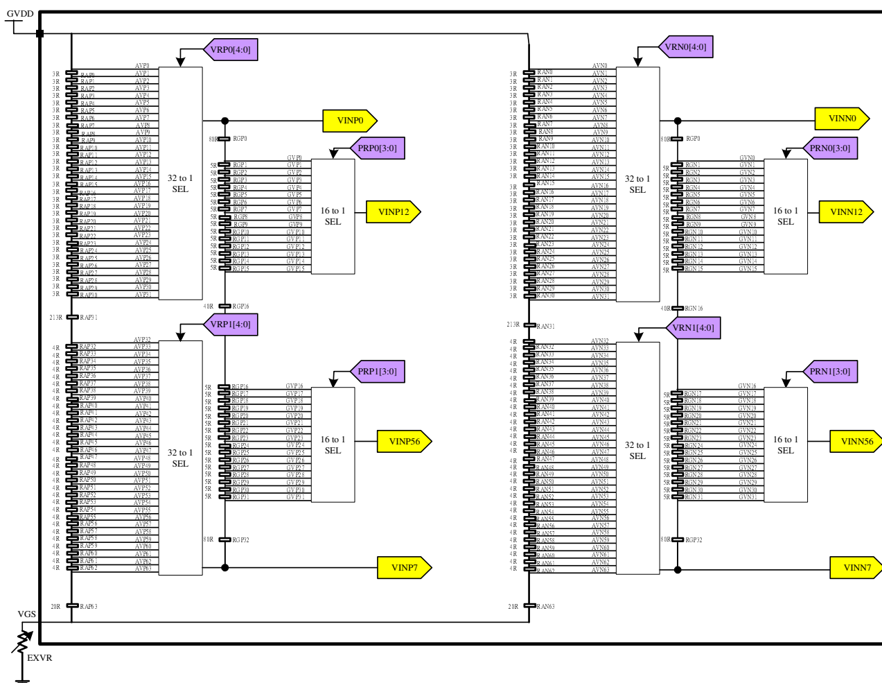
Figure37 Grayscale Voltage Adjustment 1
