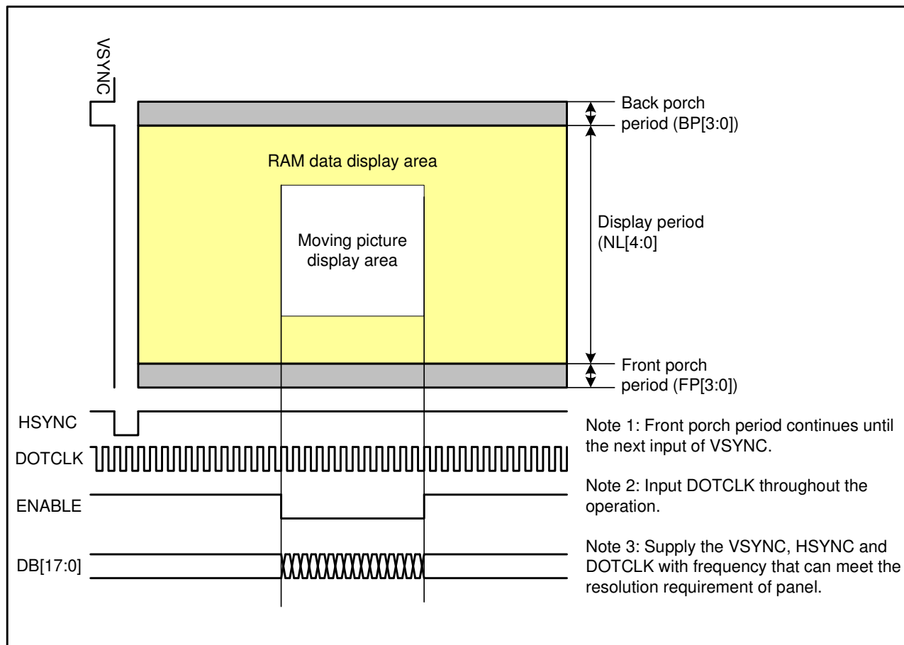
Figure13 GRAM Access Area by RGB Interface
