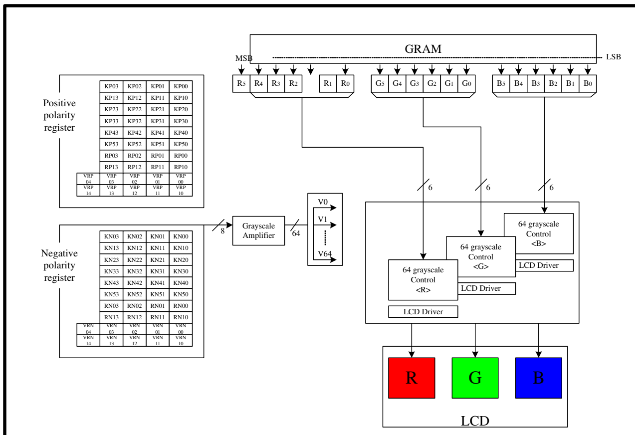
Figure35 Grayscale Mapping
