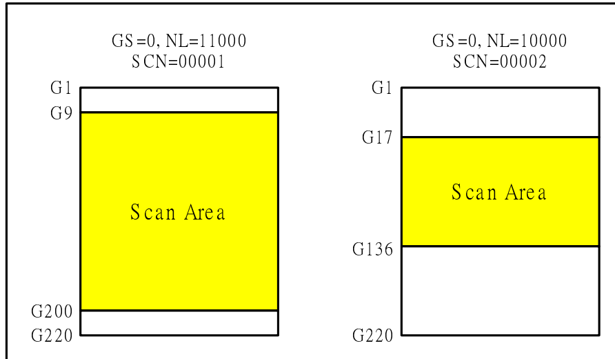
Figure28 Scanning Start Position for Gate Driver
