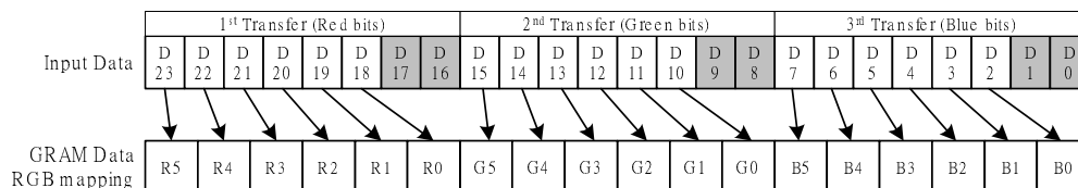
Figure9 Data Format of SPI Interface
