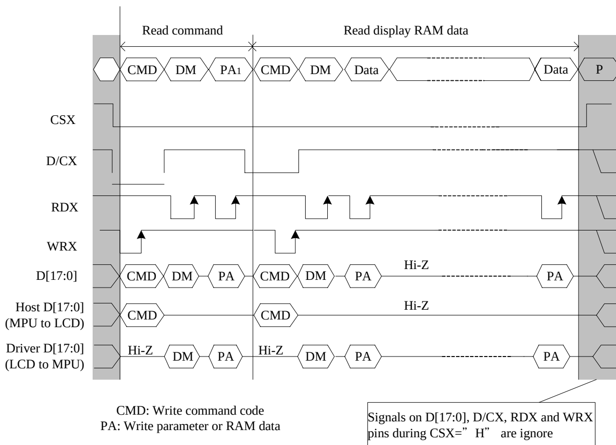
Figure16: 8080-Series parallel bus protocol (Read from register or display RAM)
