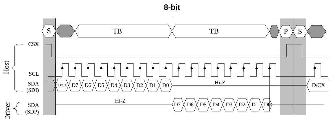
Figure7: 3-Pin Serial Protocol (for RDID1/RDID2/RDID3/0Ah/0Bh/0Ch/0Dh/0Eh/0Fh command:
