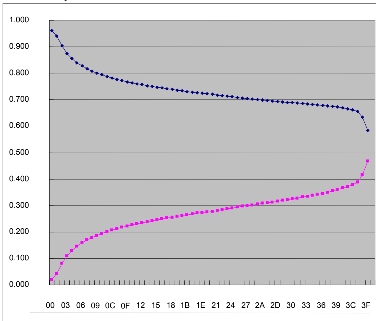
Figure 6.1: Gamma curve
