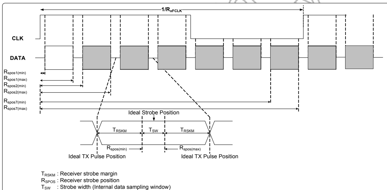
Figure 10.1: LVDS figure
