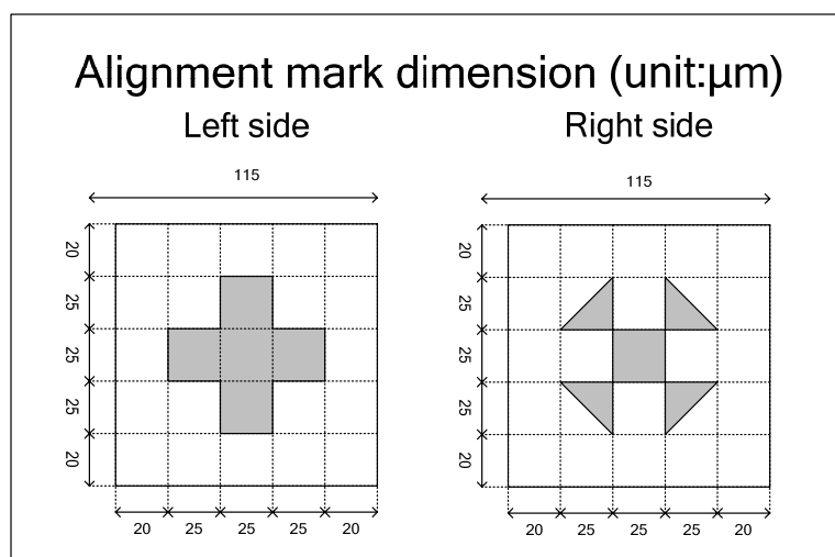
Figure 12.3: Alignment mark
