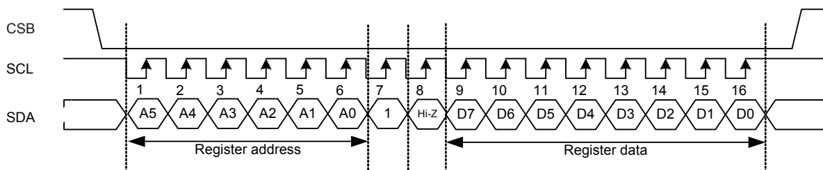
Figure 7.3: Read format
