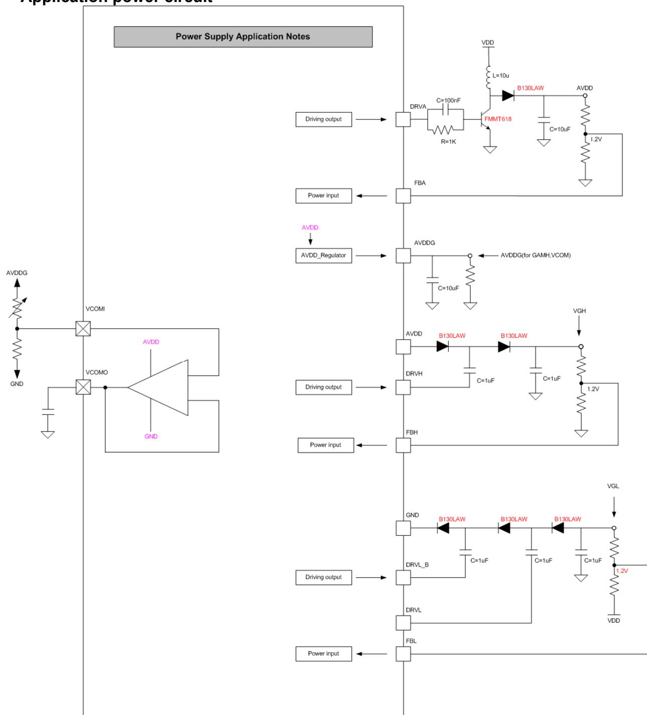
Figure 3.6: Application power circuit
