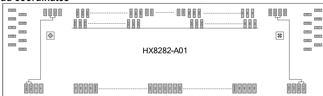
Figure 12.4: Pad coordinate
