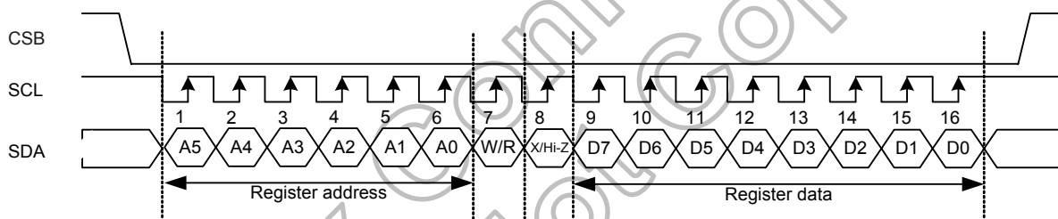
Figure 7.1: SPI format
