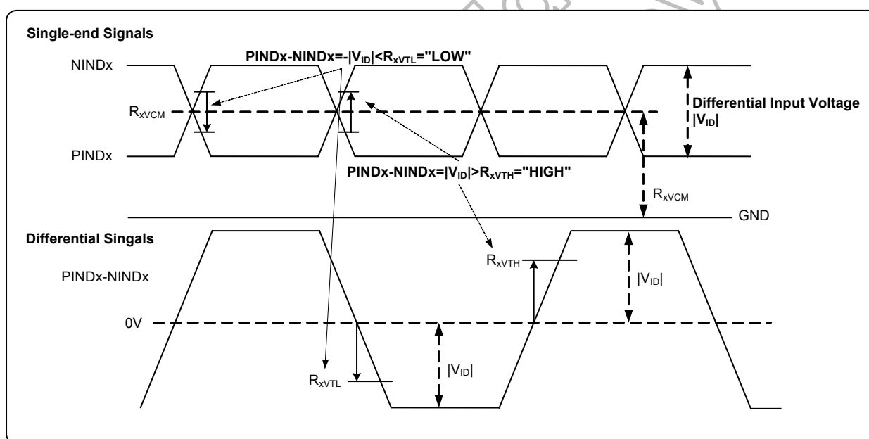
Figure 9.1: Single-end signals
