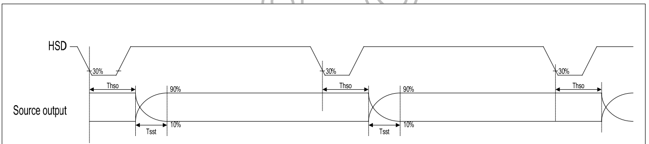
Figure 10. 2 Source Output Timing Diagram
