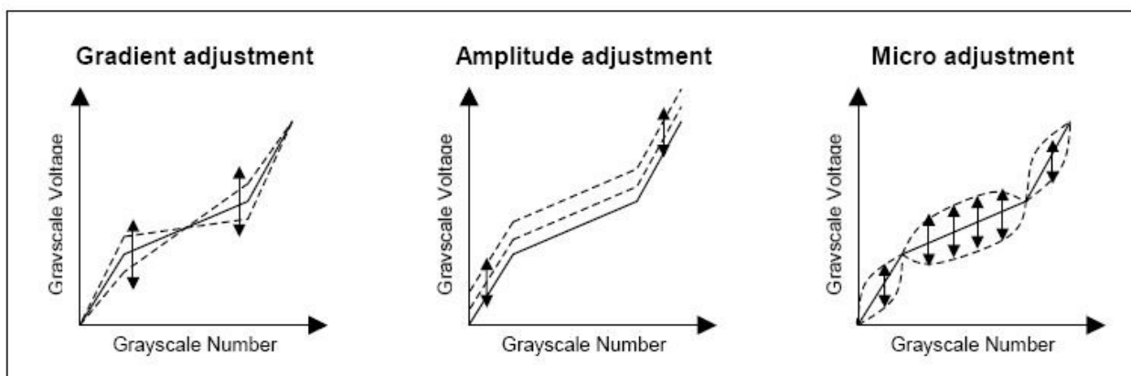
Fig 13. Gamma Adjustment Function
