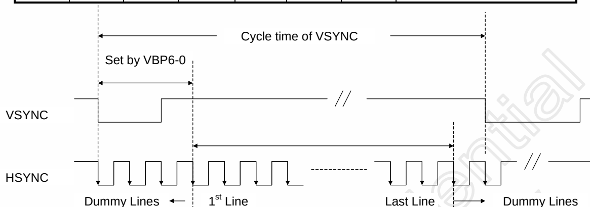
Fig 20. Vertical data
