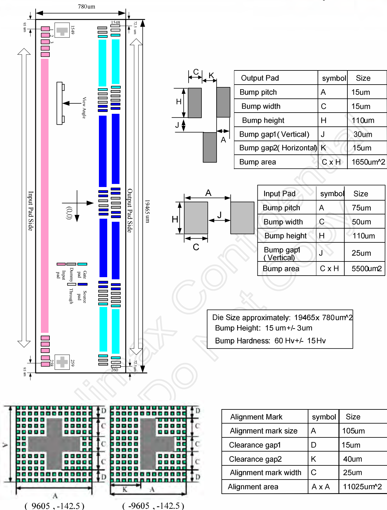
Fig 2. HX8257-A Die Floor Plan (Bump Face UP)
