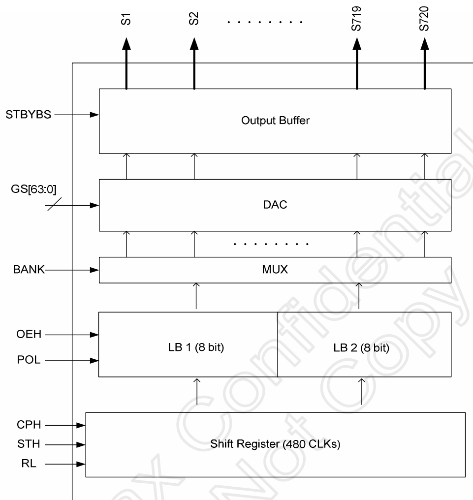
Fig 8. Source Block
