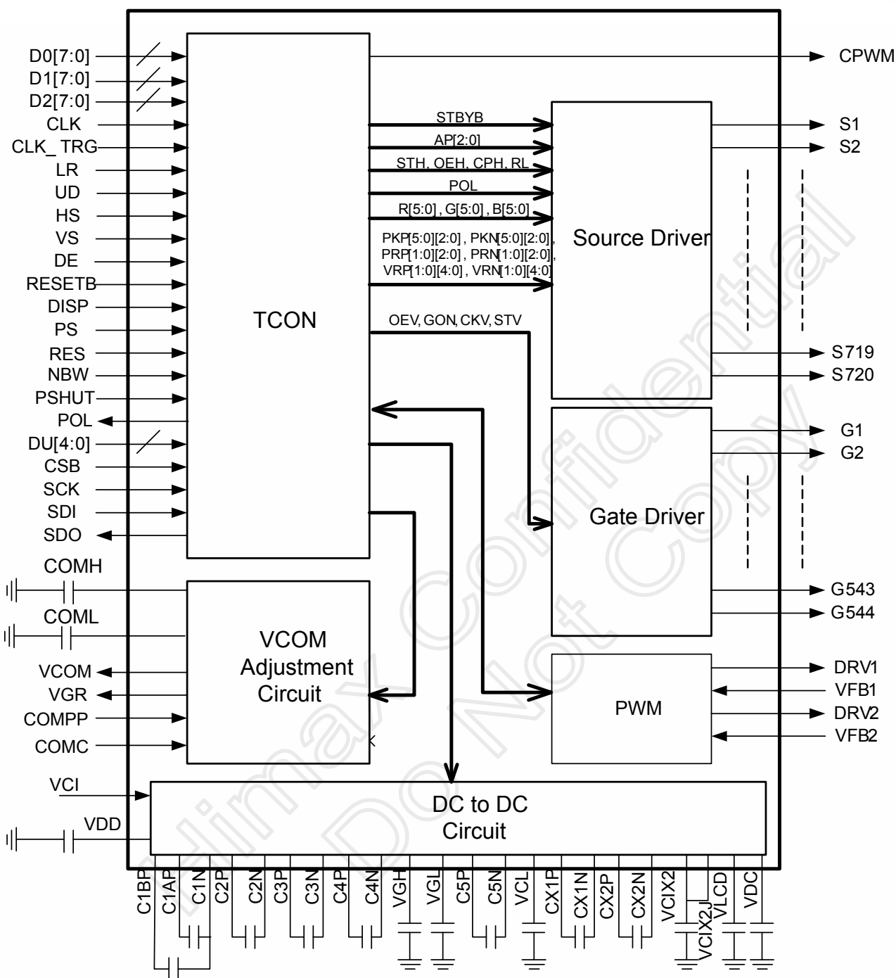
Fig 1. Block diagram
