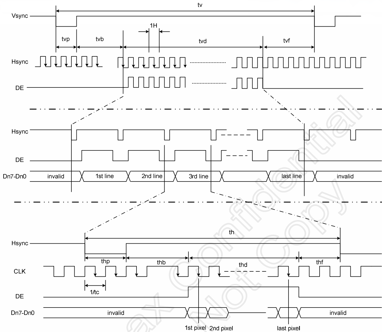
Fig 23. Parallel RGB input timing
