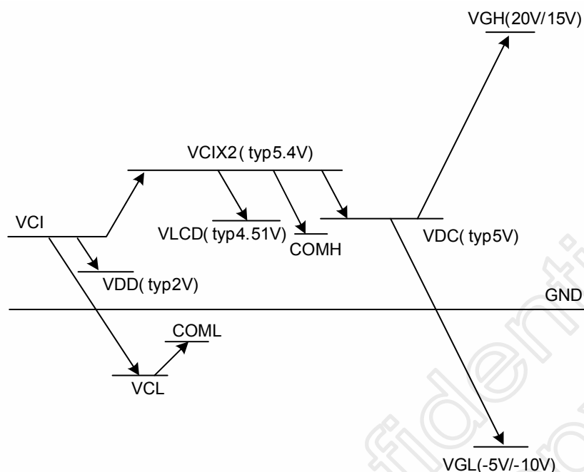
Fig 3. Power Block
