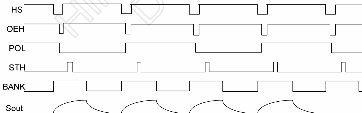
Fig 9. Source Sequence
