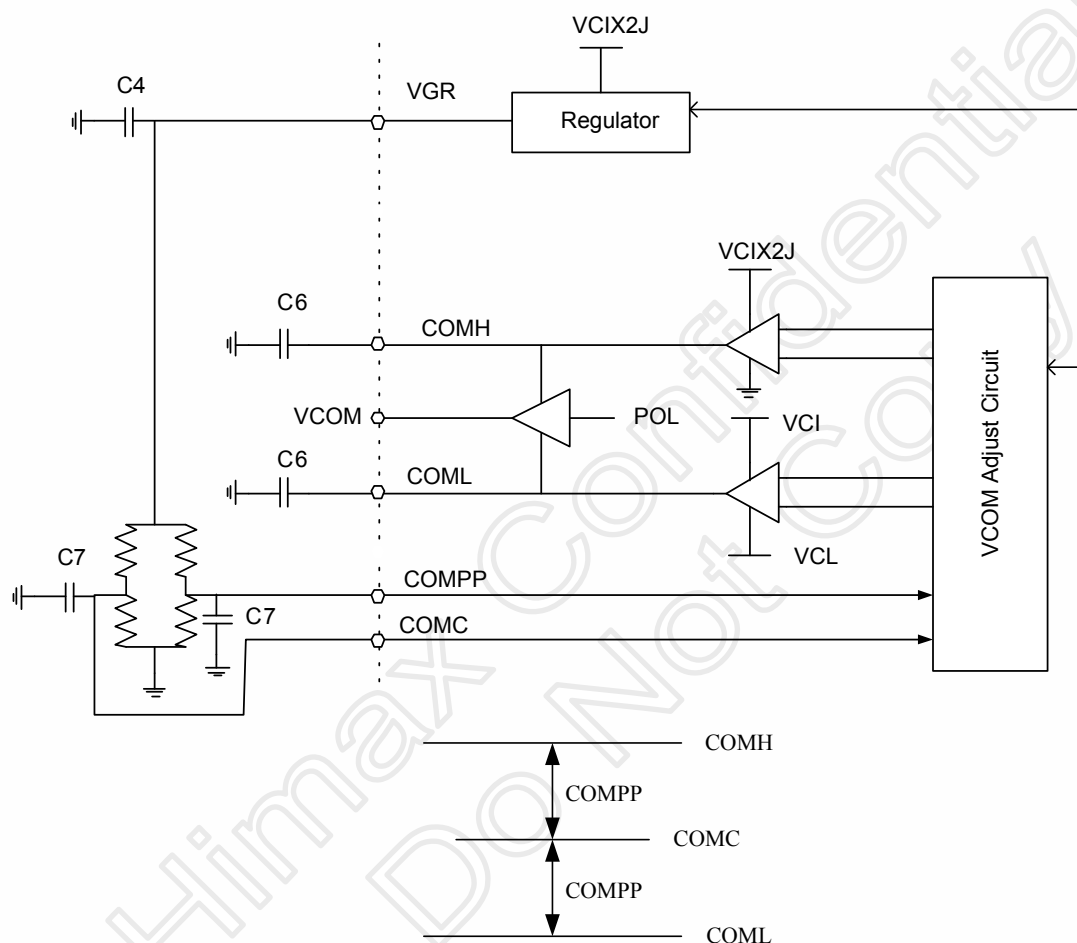
Fig 5. VCOM Block
