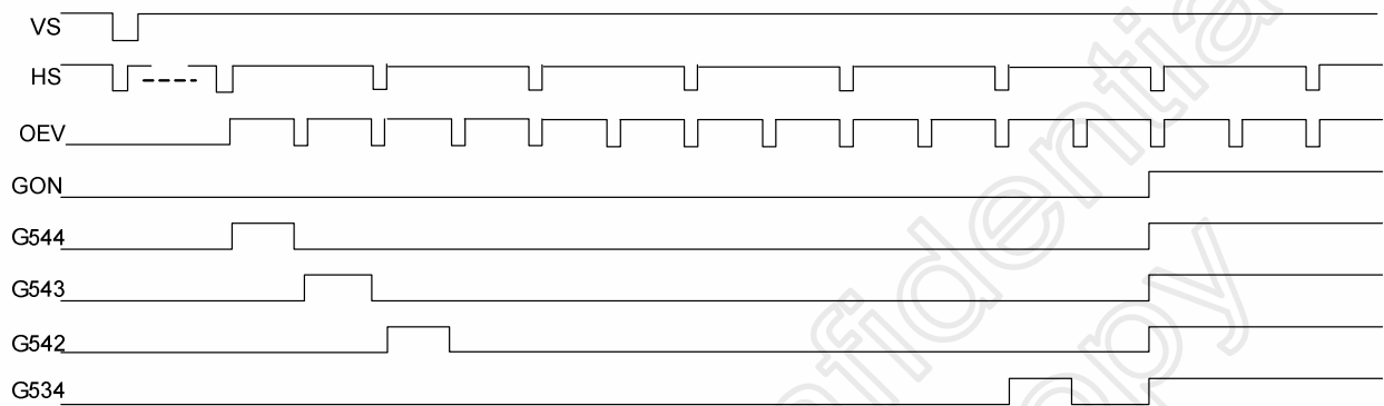
Fig 7. Gate Sequence
