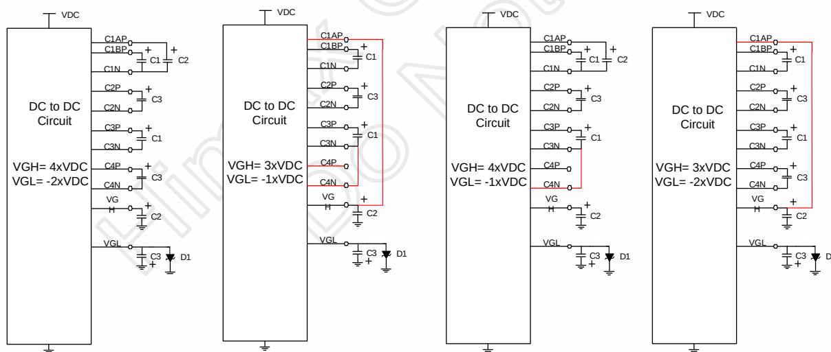
Fig 4. VGH/VGL External Setting
