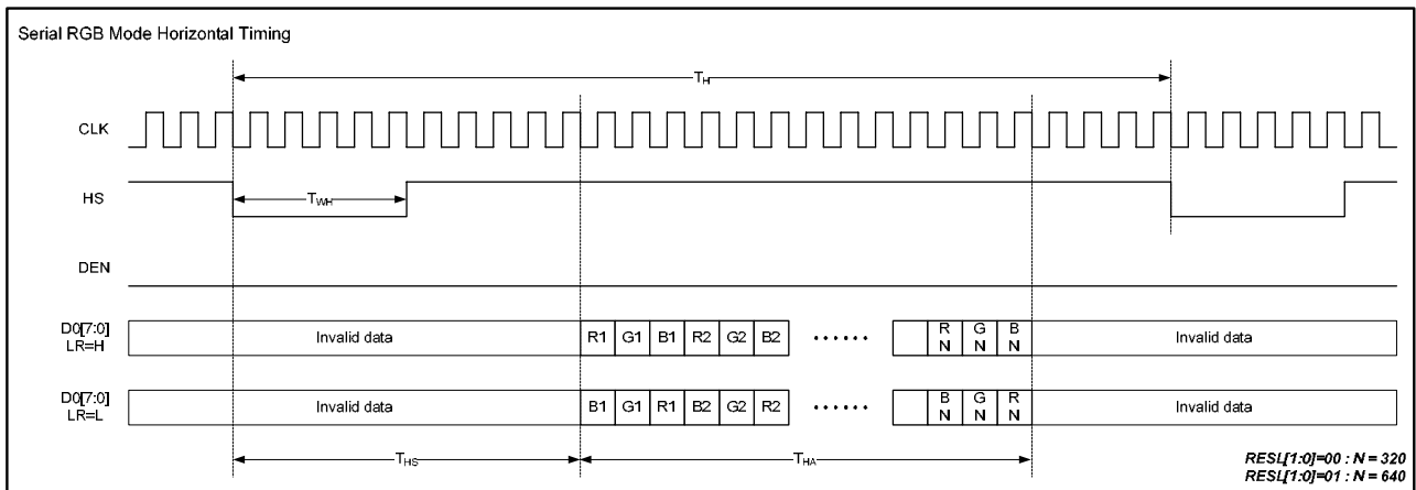
Figure 8. 2 Serial RGB SYNC Mode Horizontal Data Format
