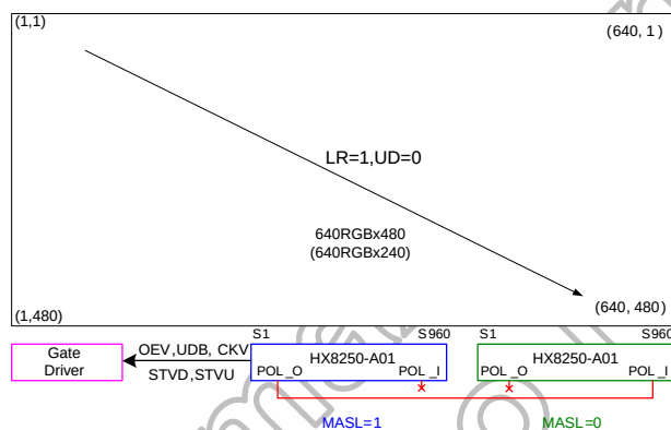
Figure 5. 5 2-chip cascade for 1920x480
