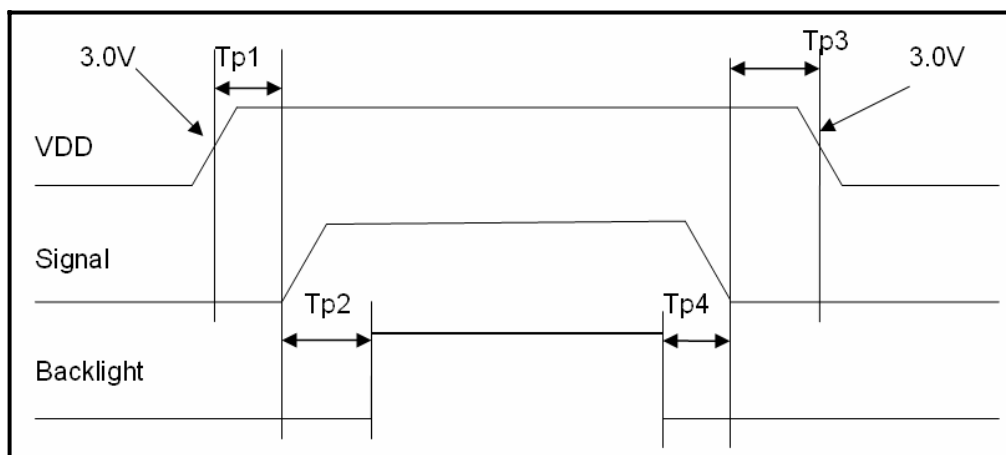
Figure 1.2 Interface power on/off sequenc
