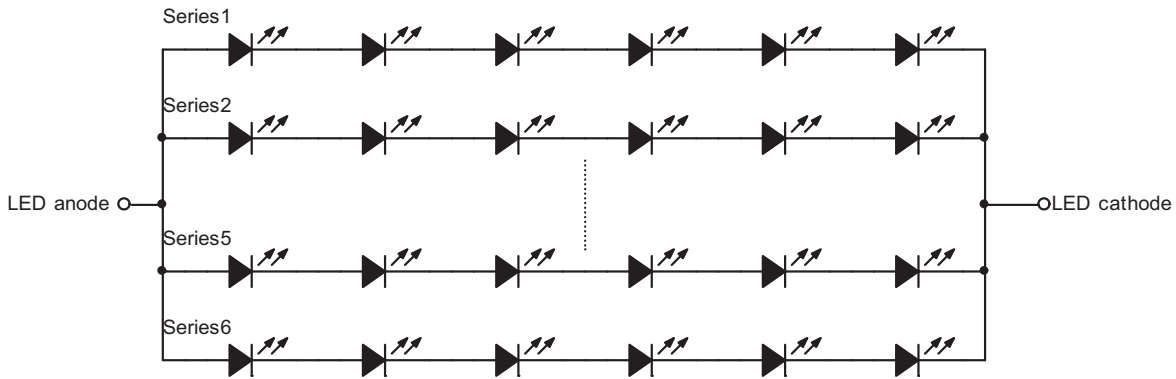
Figure 2. LED connection of backlight
