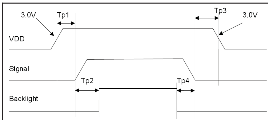
Figure 2. Interface power on/off sequenc
