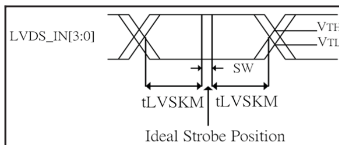
SW: Setup and Hold time Figure 1. Input signal data timing
