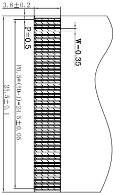
DETAIL A 5:1
