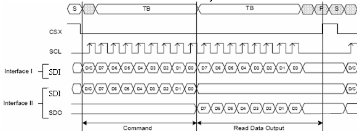
Figure.1-53-Wire9-BitSerialInterface/IIBusProtocol,Read1-ByteFromRegister
