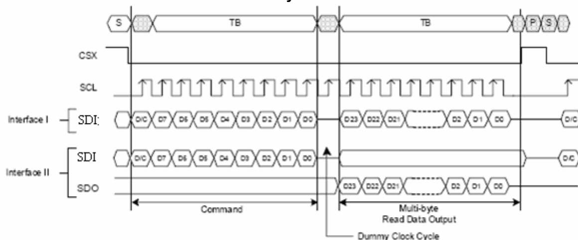
Figure.1-63-Wire9-BitSerialInterface/IIBusProtocol,Read3-ByteFromRegister
