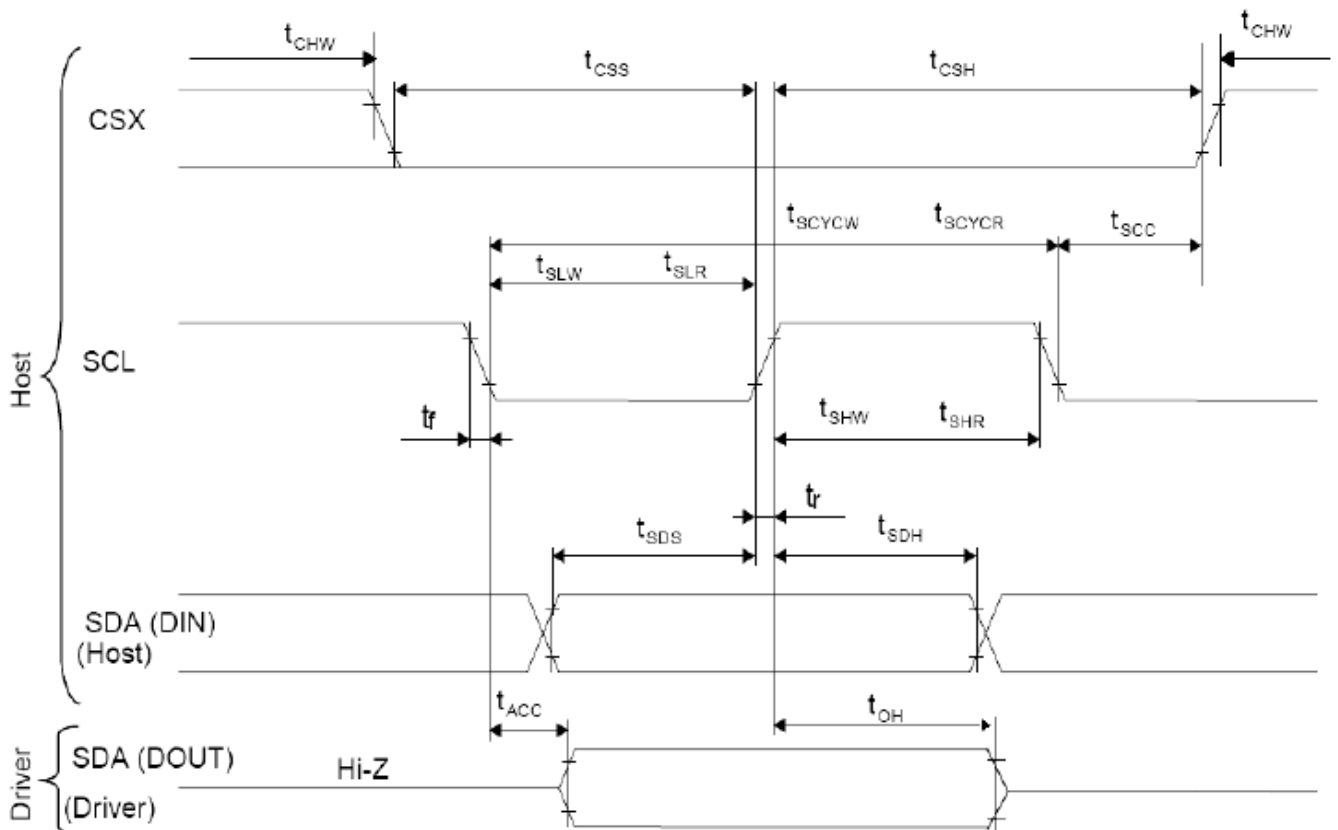
Fig.1-7ACCharacteristicsof3-Wire9-BitSerialInterfacetiming
