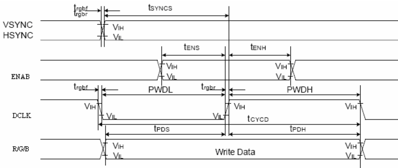
Fig.1-1RGBInterfaceTiming
