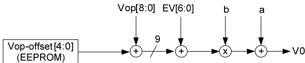
Figure 7.9-4 V0 value control for different modules by loading EEPROM offset
