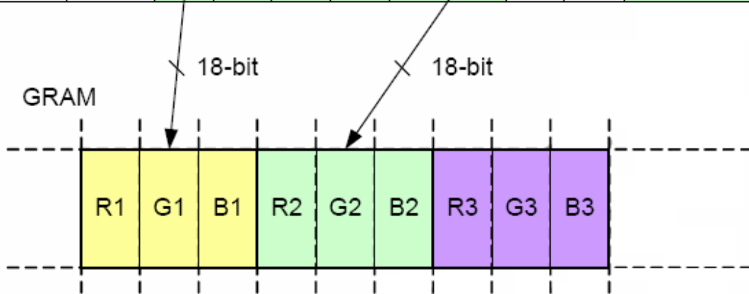
Figure 5.4.1 8-bit Data Bus GRAM Write/Read Data Format(262K)
