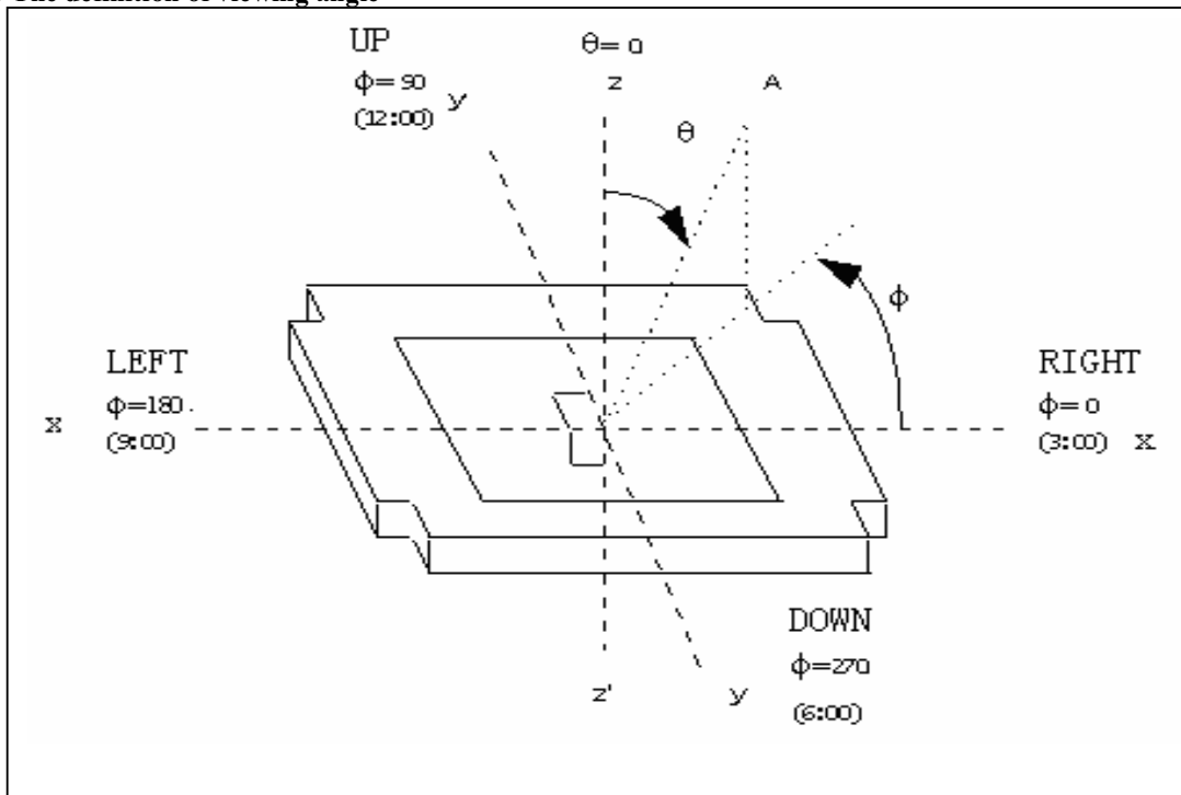
FIG. 3 The definition of viewing angle
