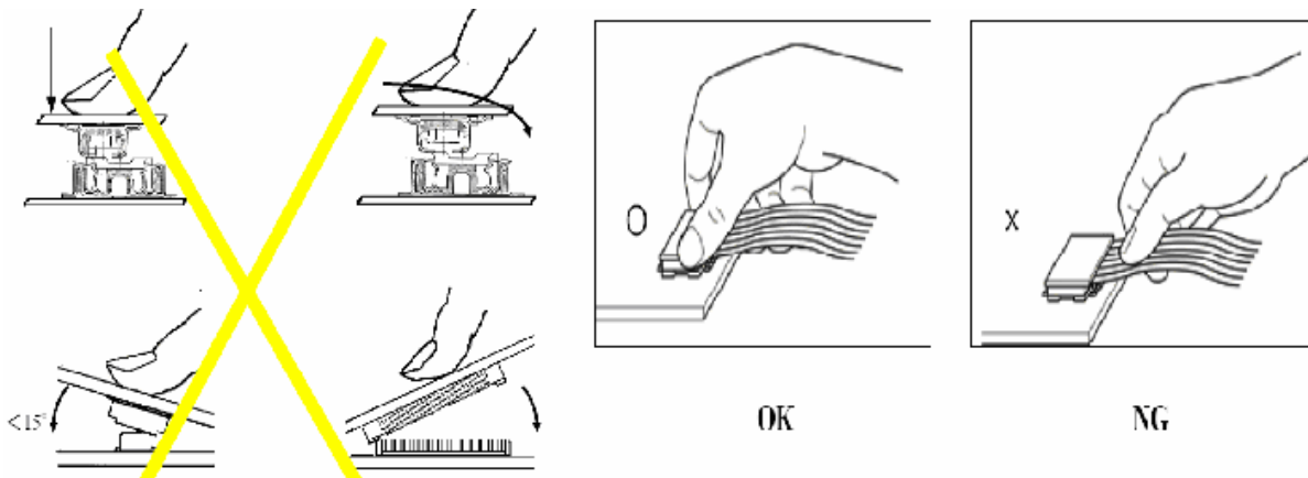
Precaution for soldering the LCM
