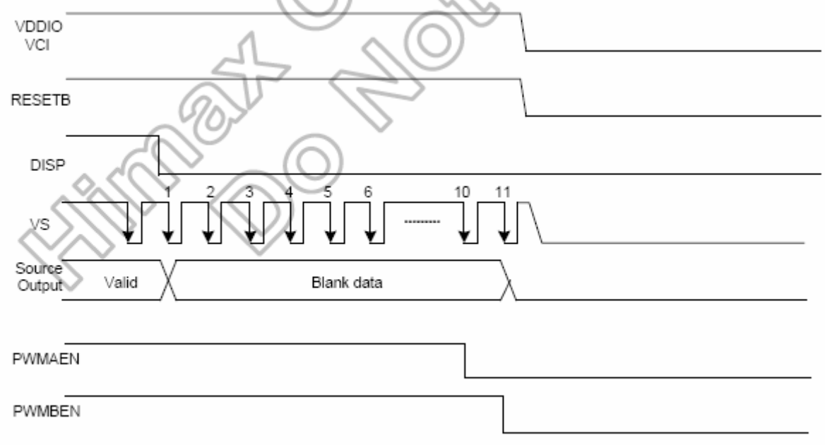
Figure 7.15 Power Off Sequence
