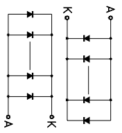
1. LED CIRCUIT DIAGRAM: (LED M3882=76 Dips) Color: YELLOW-GREEN
