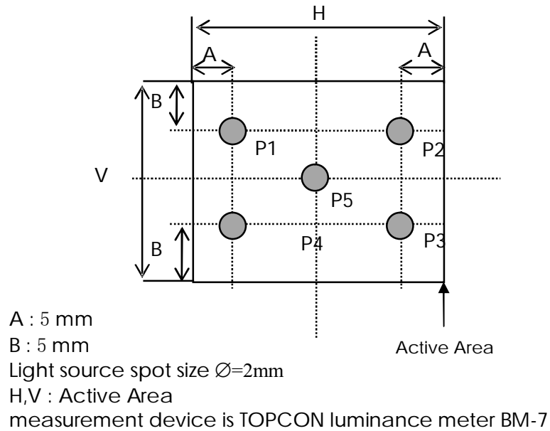
FIG. 5 The definition of viewing angle
