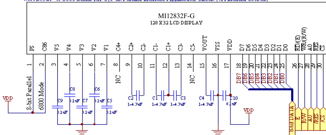
MI12832F-G 6800 Series MPU, 8-bit Parallel Interface Application Circuit (4X internal booster)
