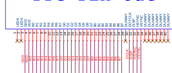
FPC Pin Out
