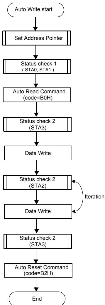
Fig.20 Flowchart for Data Auto Read/Write mode
