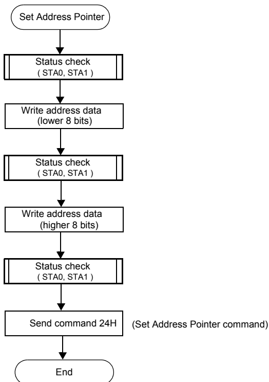
Fig.11 The flowchart for programming Address Pointer Register
