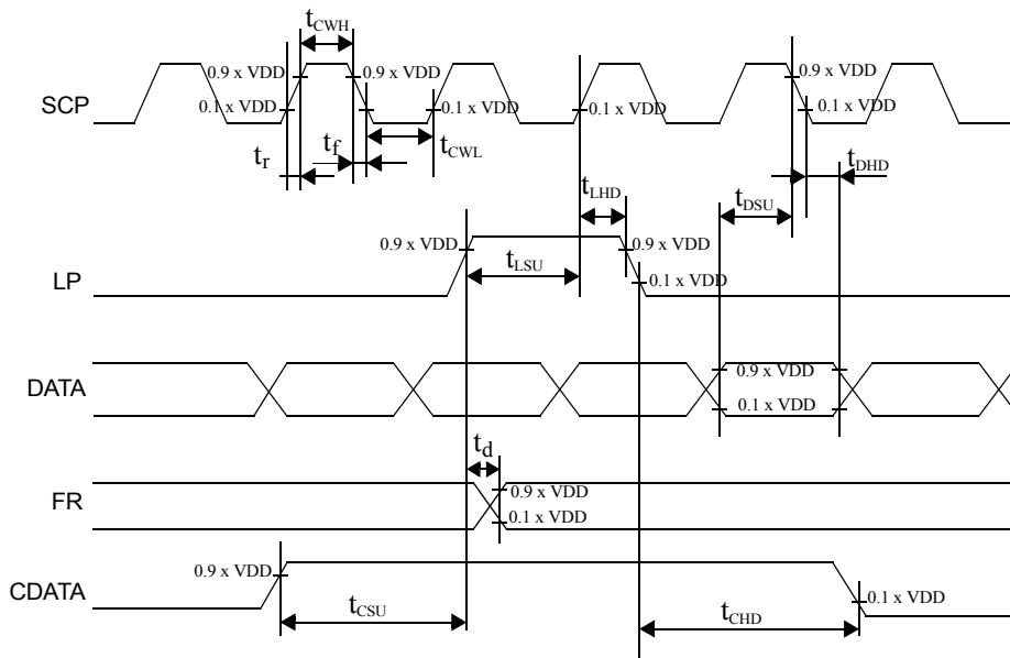
Fig.25 Driver clock characteristics
