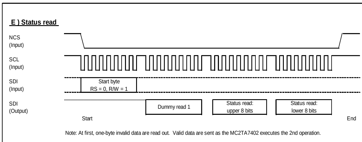
Figure 14-14: Data transmission through SPI (2)
