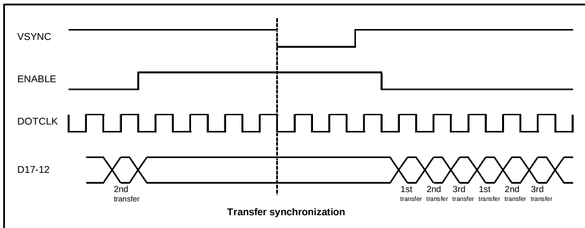
Figure 16-7: 6-bit data transfer synchronization
