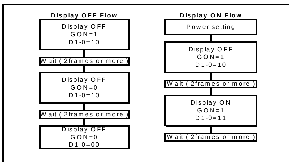
Figure 25-1: Display ON/OFF flowchart
