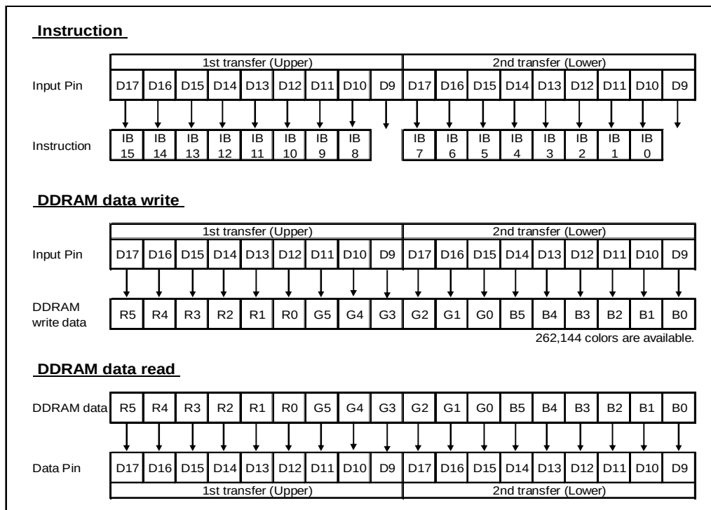
Figure 14-6: Data format for 9-bit interface
