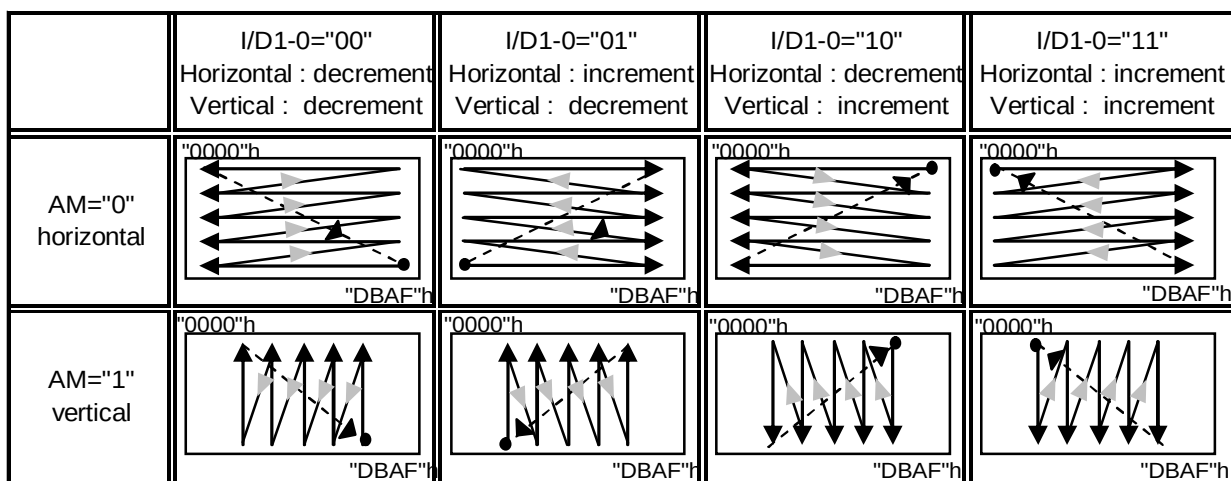
Figure 10-4: Address transition directions
