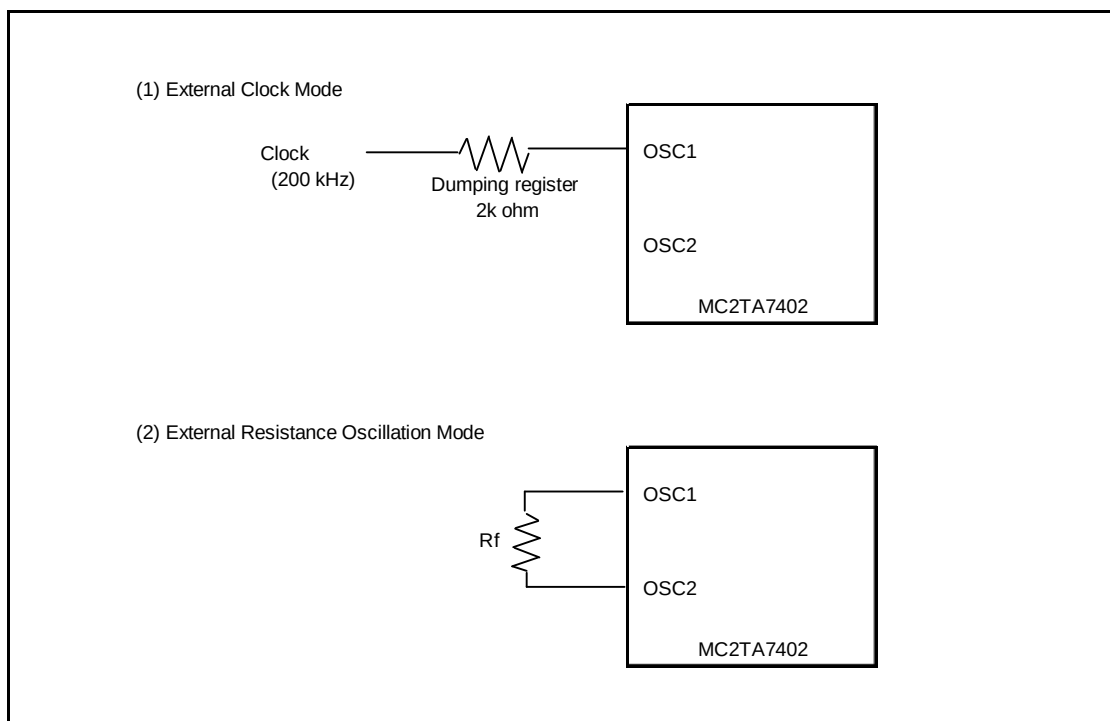
Figure 27-1: Oscillation Circuit
