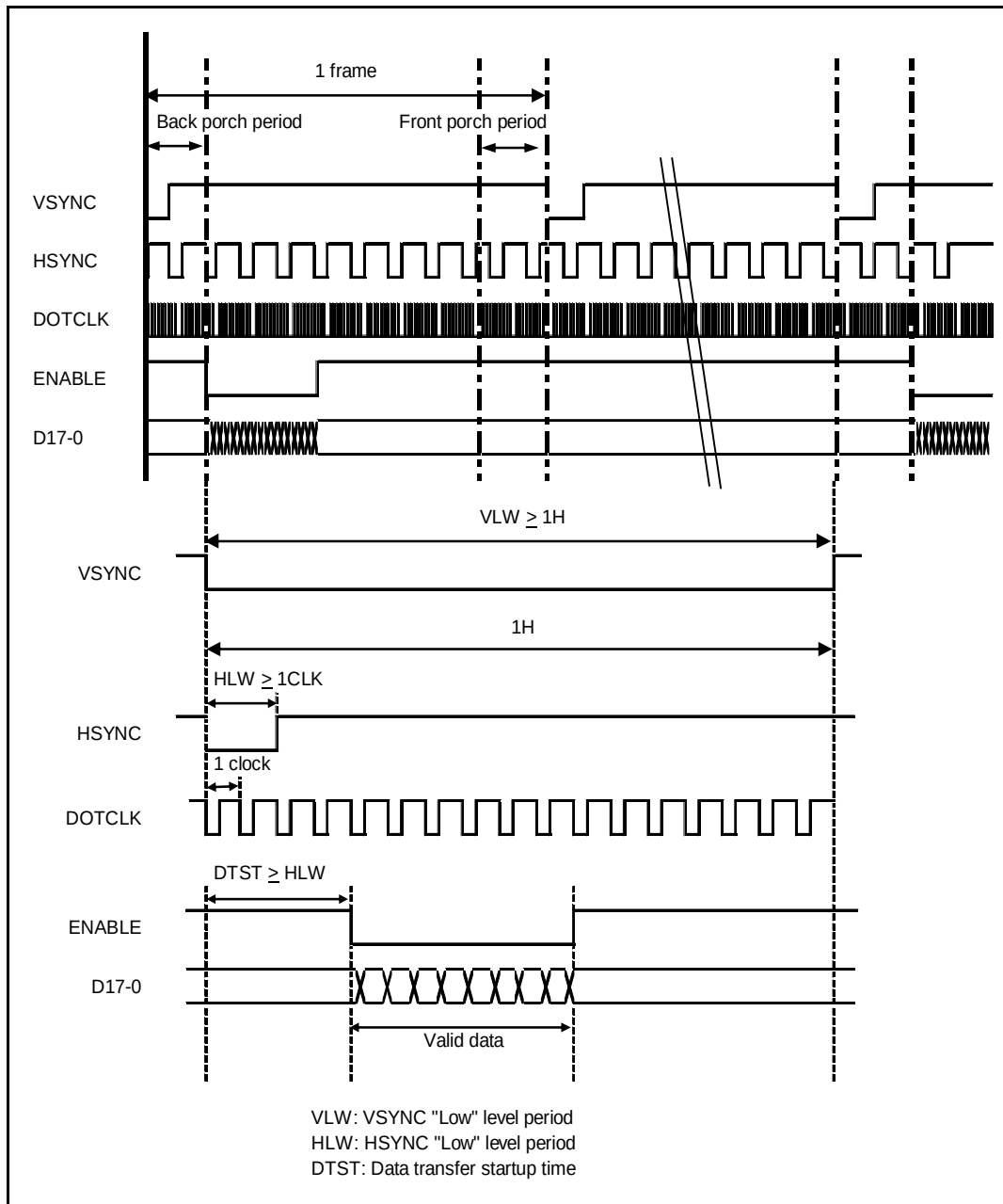
Figure 16-2: 16-/18-bit RGB Interface Timing
