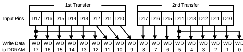
Figure 8-1: Input pins and DDRAM write (System Interface) -1
