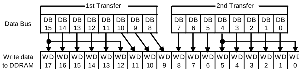
Figure 8-3: Input pins and DDRAM write (Serial Peripheral Interface (SPI))
