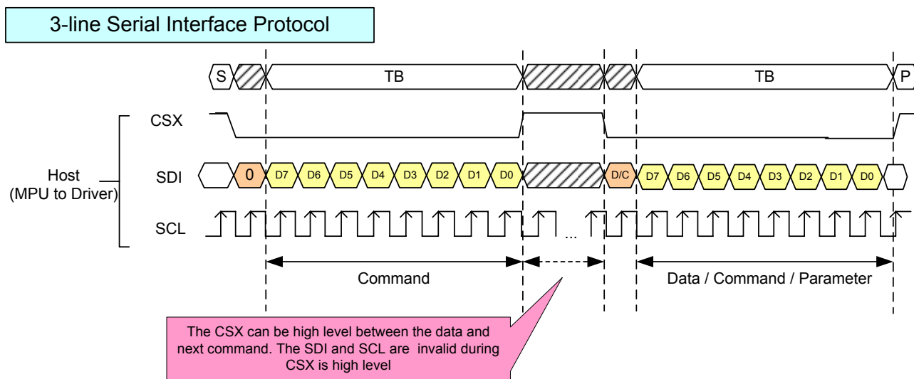
Figure 3 SPI protocol (SCL rising edge example)
