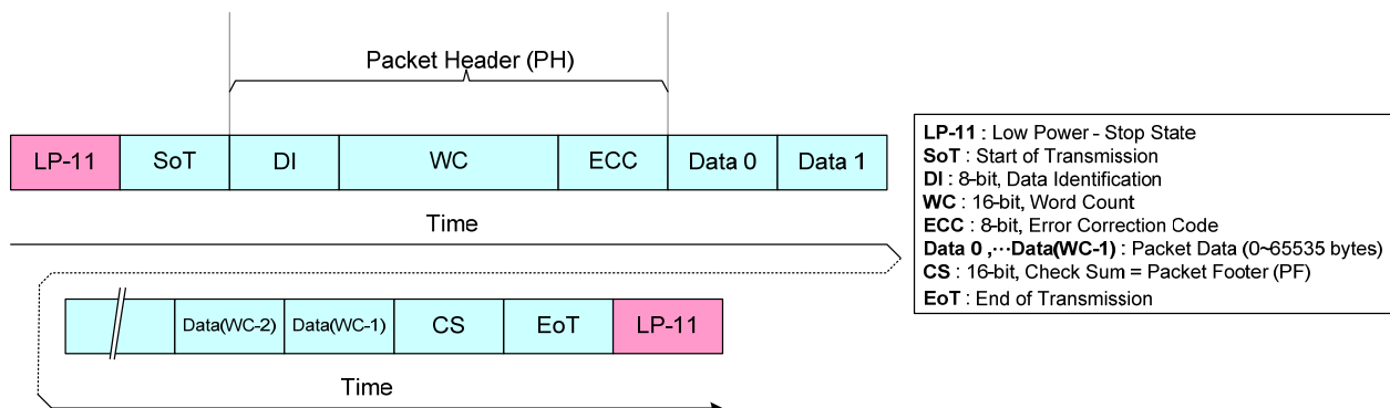
Figure 42 Long Packet (LPa) Structure
