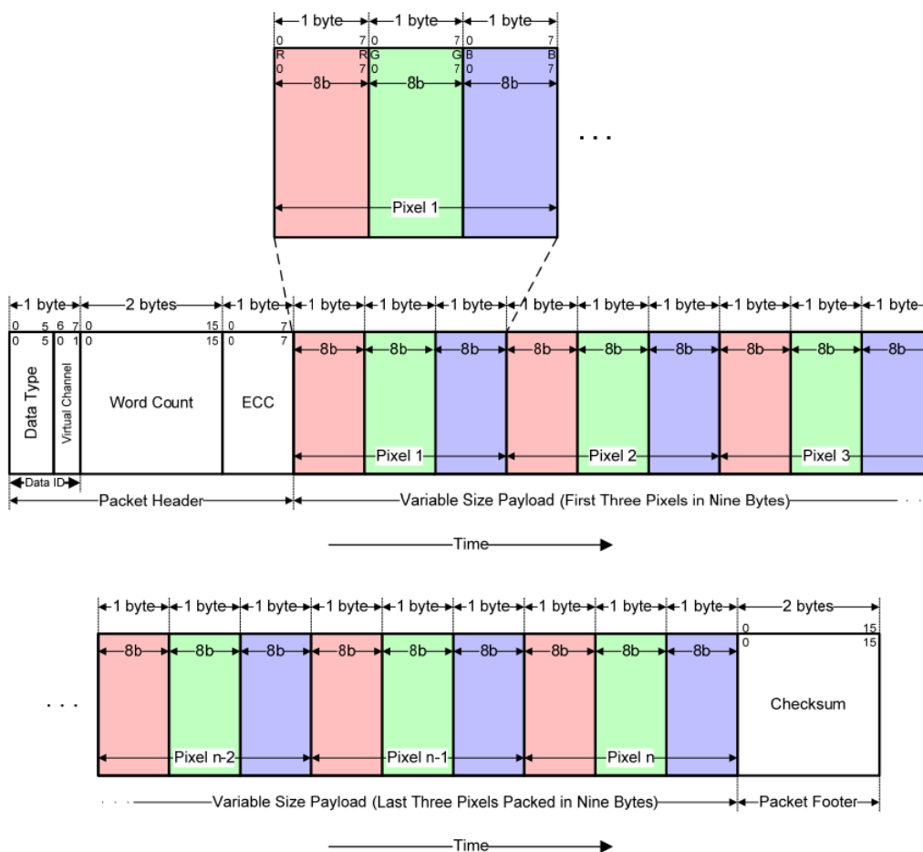
Figure 92 24-bit per Pixel, Data Type = 11 1110 (3Eh)
