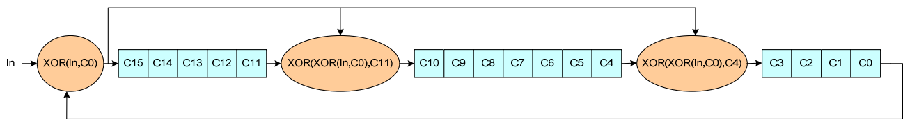
Figure 63 16-bit Cyclic Redundancy Check (CRC) Calculation
