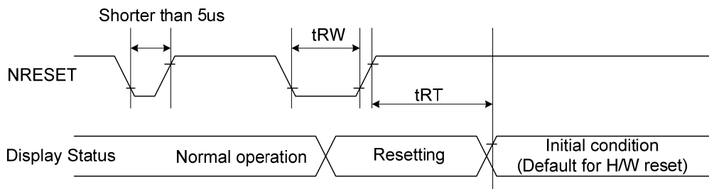
Figure 102 Reset Timing
