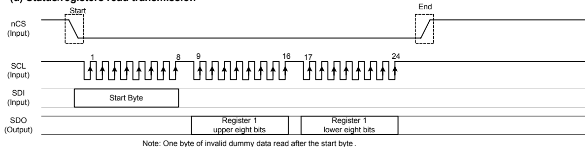
Figure8 Data transmission through serial peripheral interface (SPI)
