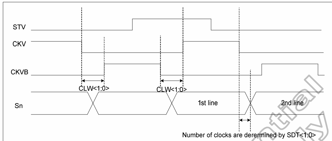
Figure 7. 24 CLW Bits
