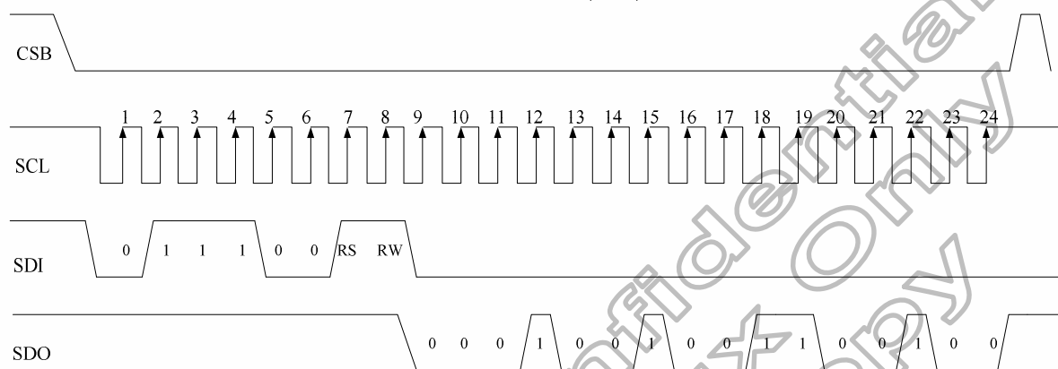
Figure 12. 13 (b) SPI interface Timing Diagram & Read SPI Example
