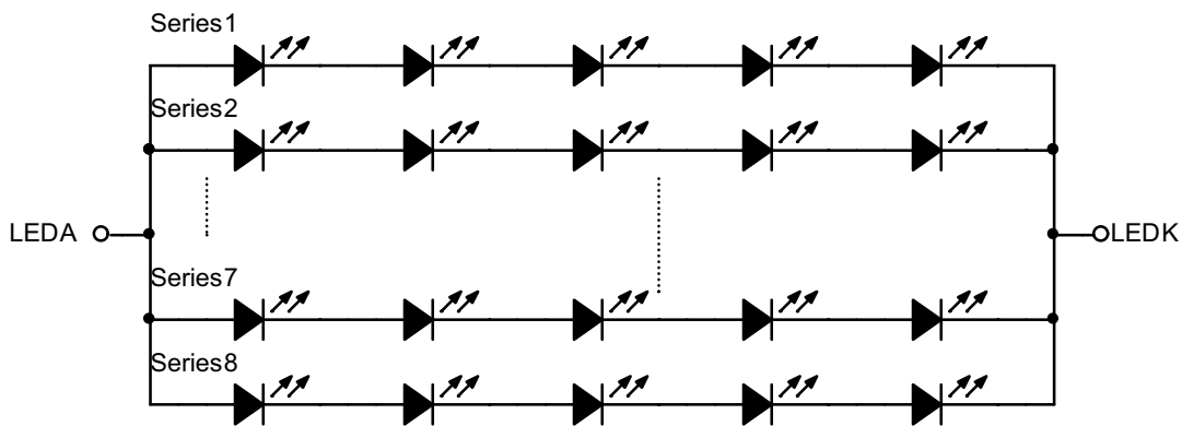
LED connection of backlight
