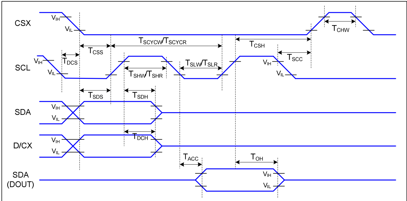
Figure 1.1: 4-line serial interface timing Ta=25 °C, IOVCC=1.65~3.3V, VCC=2.5~3.3V
