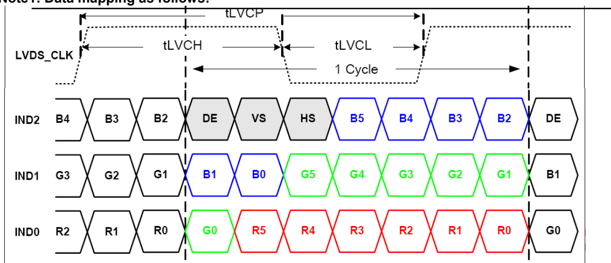
Figure 2.1 Input signal data mapping
