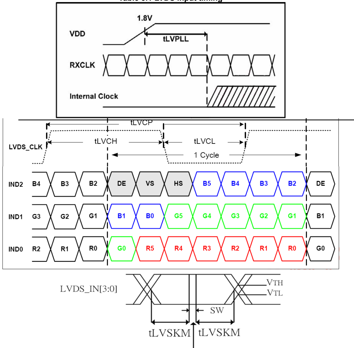
Figure 5.1 Input signal data timing
