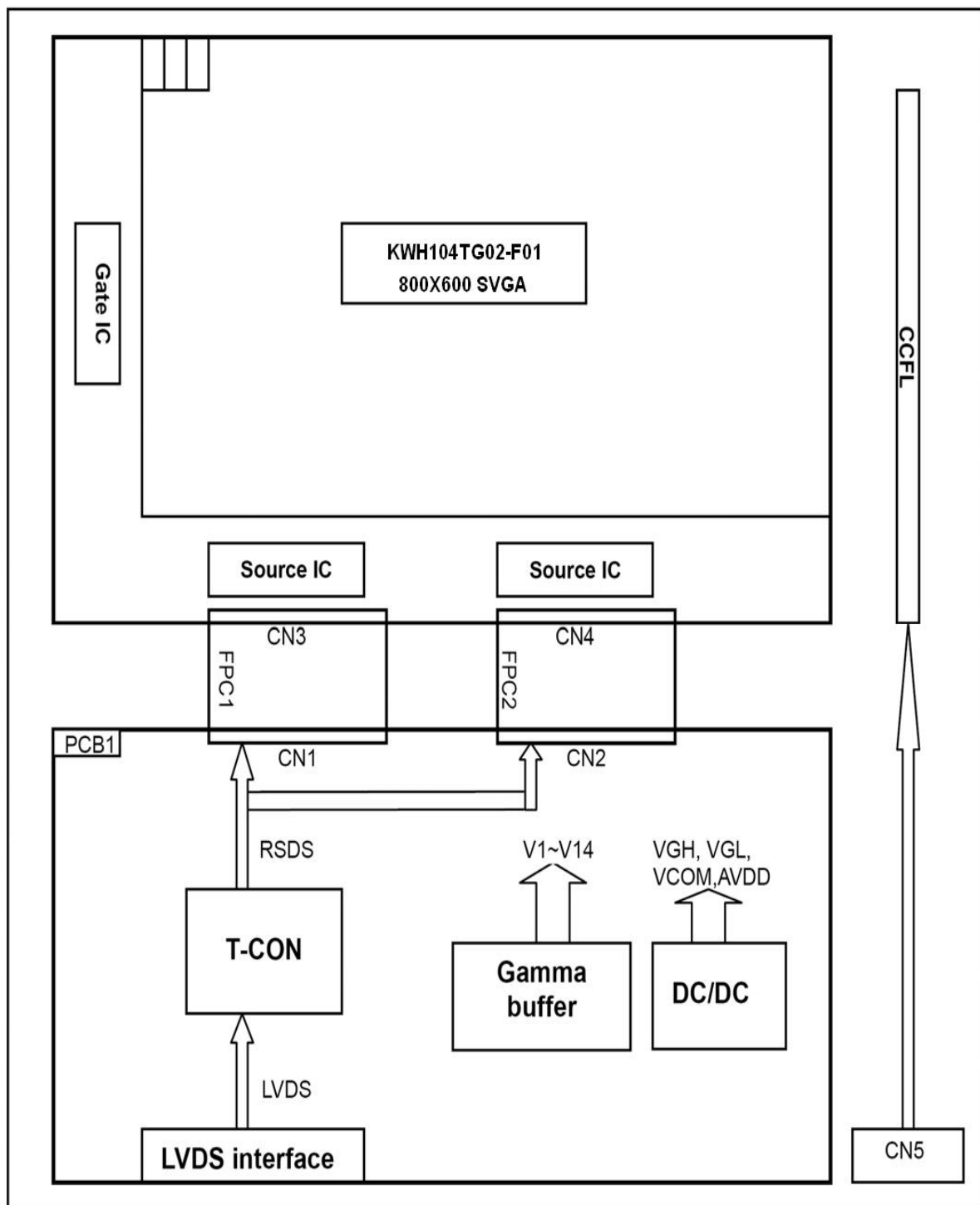
Figure 4.3 LCD module diagram
