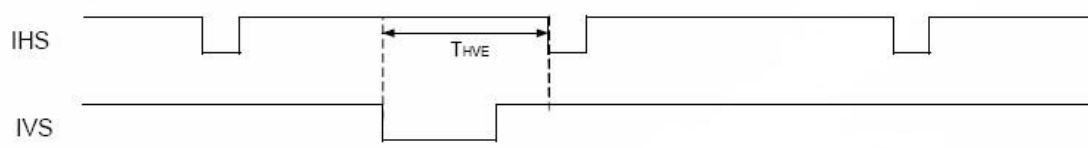
IHS and IVS waveforms in even field
