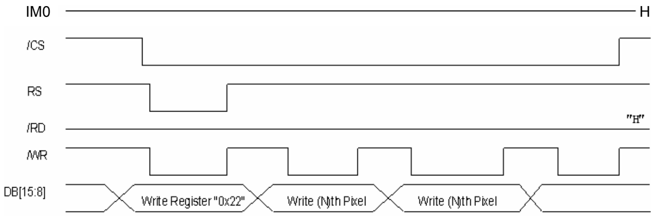
Figure 5.3.2 8-bit Write data for RGB 5-6-5-bit input (GRAM Write Timing)
