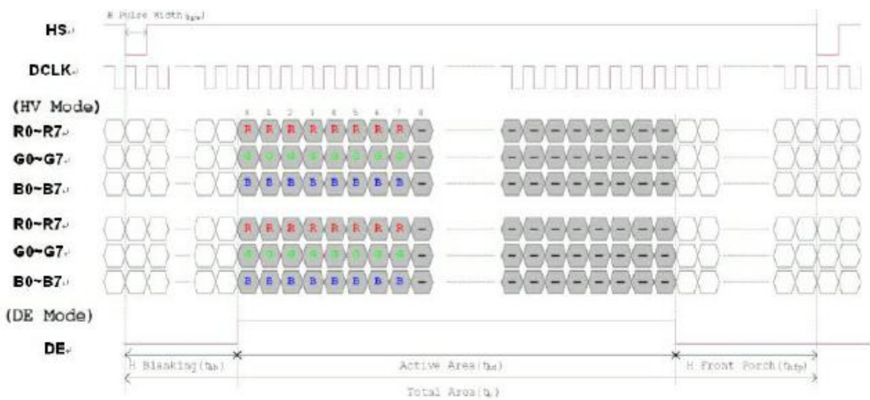
Horizontal input timing diagram.
