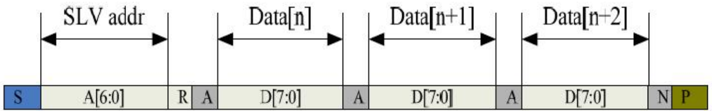
I2C master read, slave write
